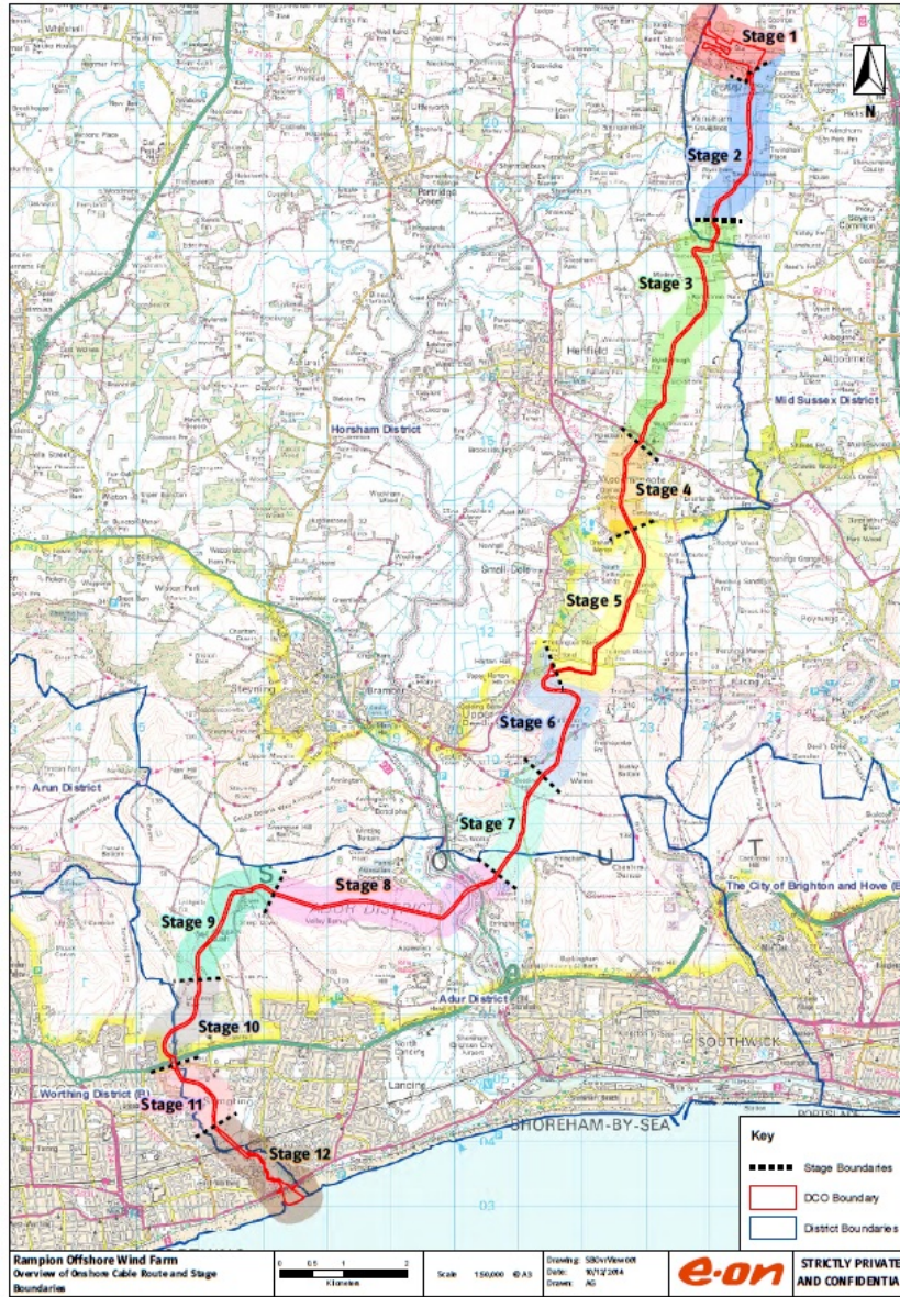
Overview Plan for Rampion 150kV Onshore Cable Route
